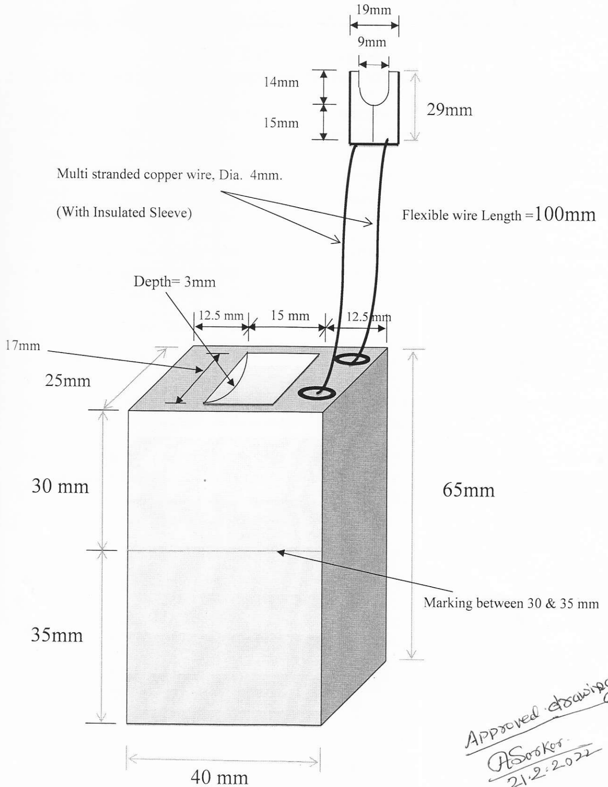
Drawing of Carbon Brush
